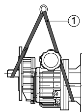
VR 1 ... VR 5.5
