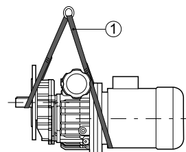
VR 0.5 ... VR 10
