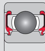
DDW Light-contact seal
