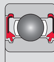
DDU Contact seal
