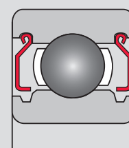
ZZ Non-contact shield
