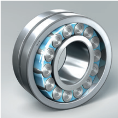
Spherical roller bearing 22311L12CAM
