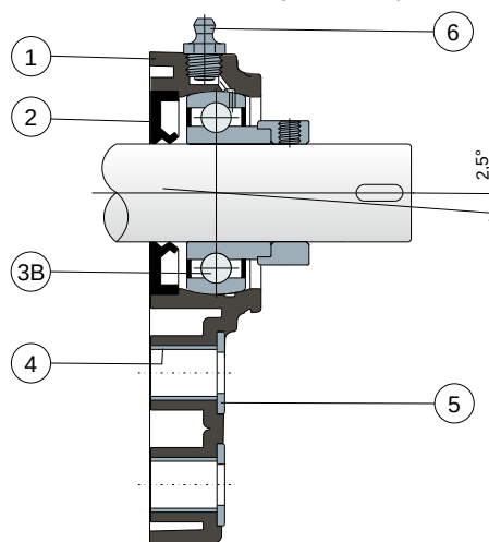
Eccentric collar shaft locking - Without protection cover
