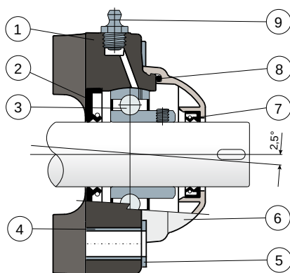
Full protection of bearing
