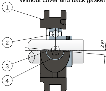
Grub screws shaft locking Without cover and back gasket
