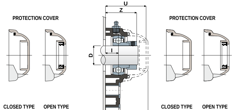
ECCENTRIC COLLAR SHAFT LOCKING
