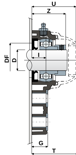
ECCENTRIC COLLAR SHAFT LOCKING
