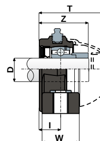
ECCENTRIC COLLAR SHAFT LOCKING
